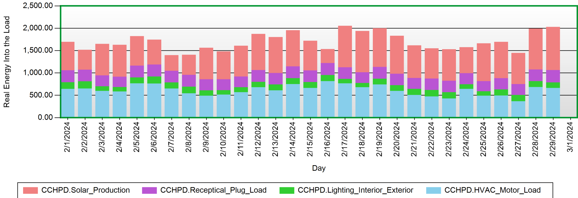
Energy Usage 00:00 - 00:00
