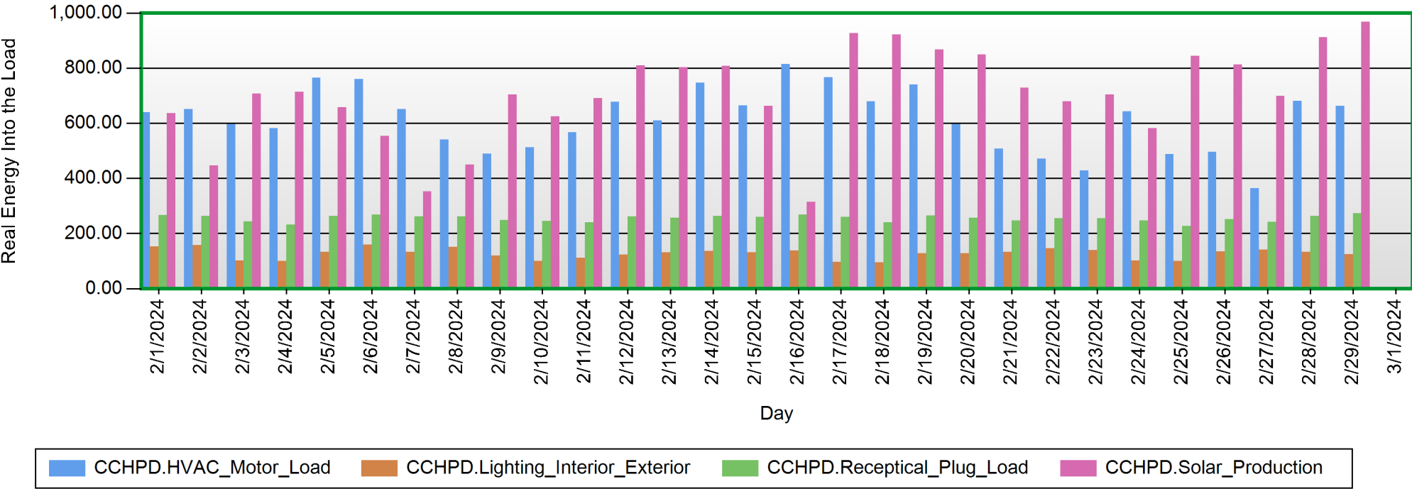
Energy Usage 00:00 - 00:00
